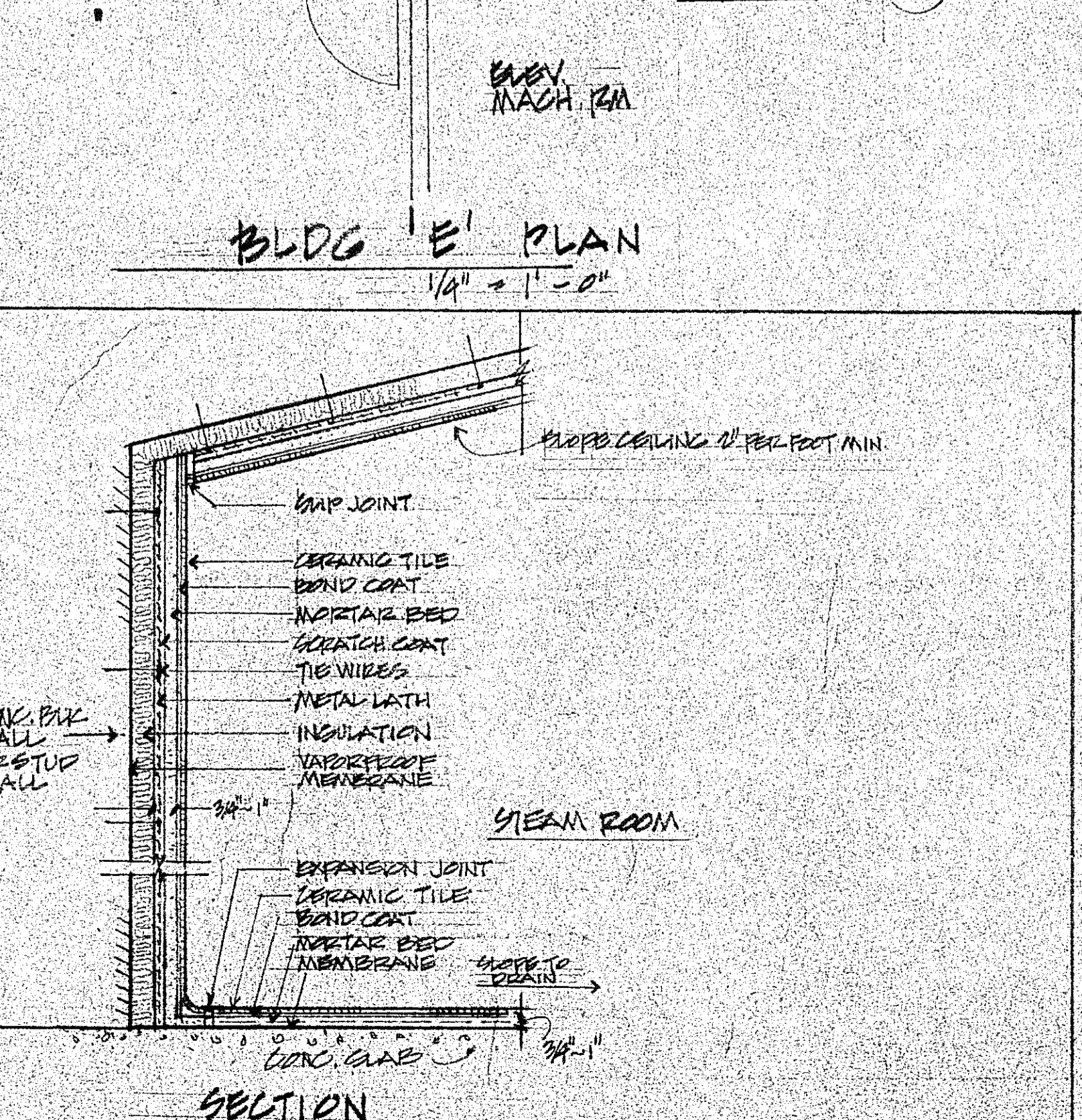
STEAM ROOM DETAIL
