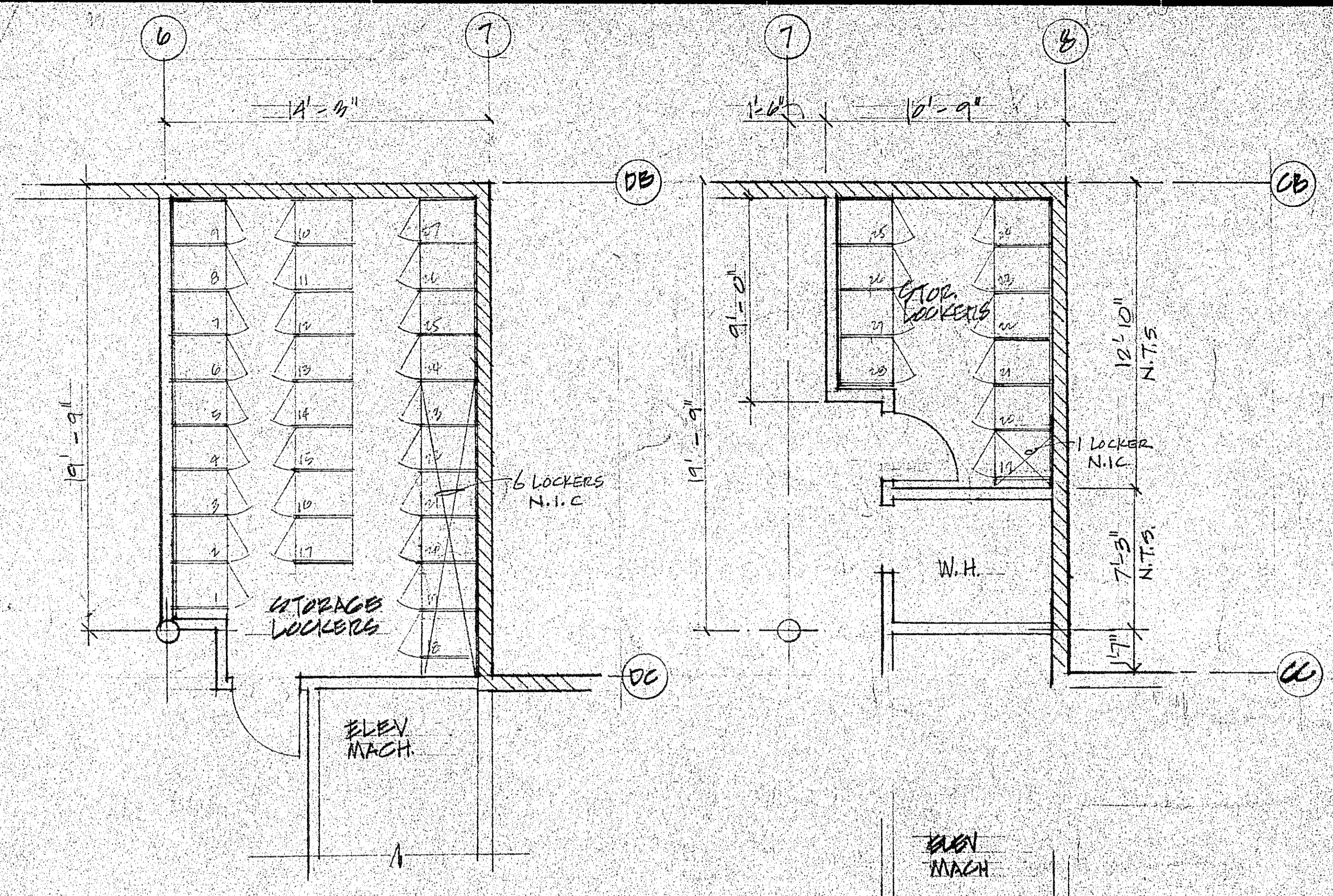
BLDG. 'D' PLAN 1/4" = 1' - 0"
