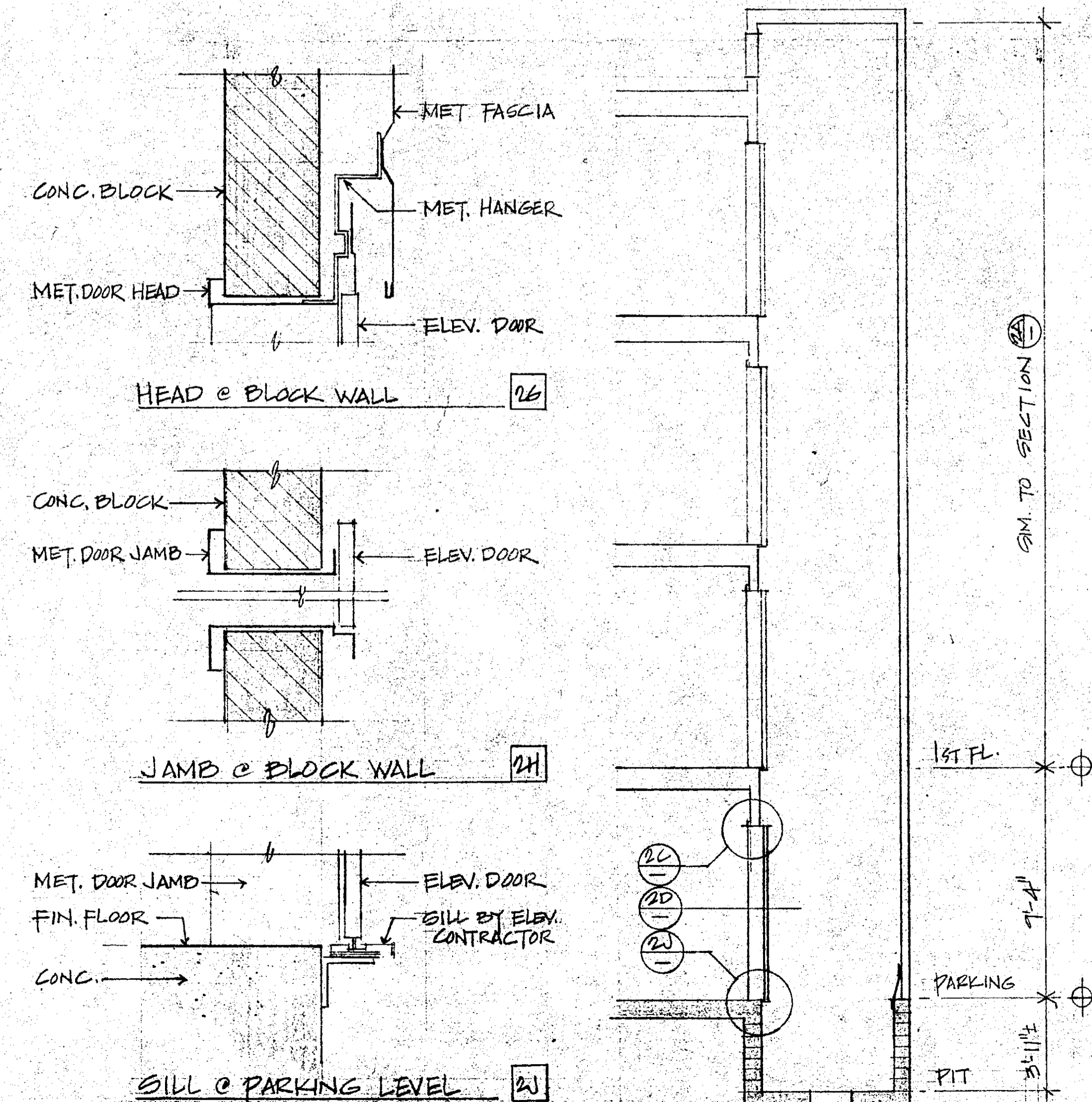
SECTION THRU ELEVATOR SHAFT 2B BLDG. "E"
