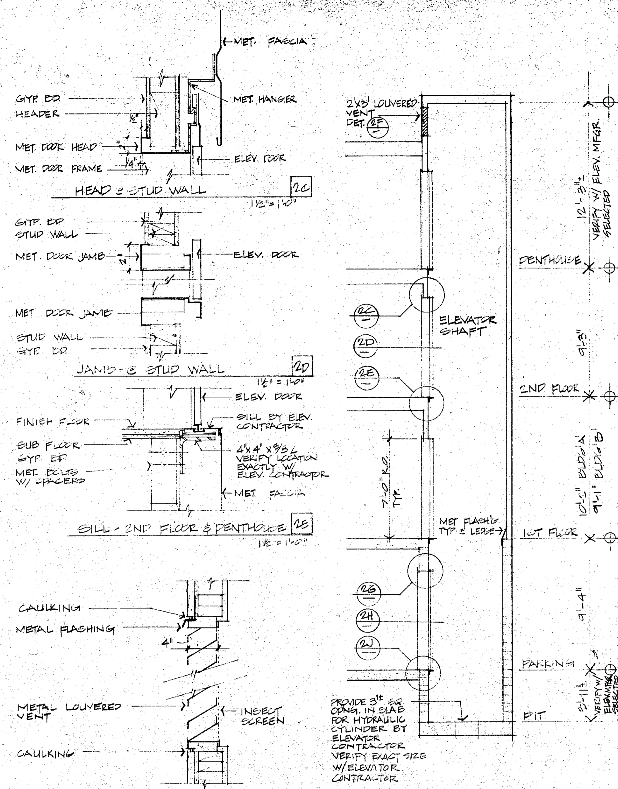
ELEVATOR SHAFT VENT 14F 1/2" = 1'-0"
