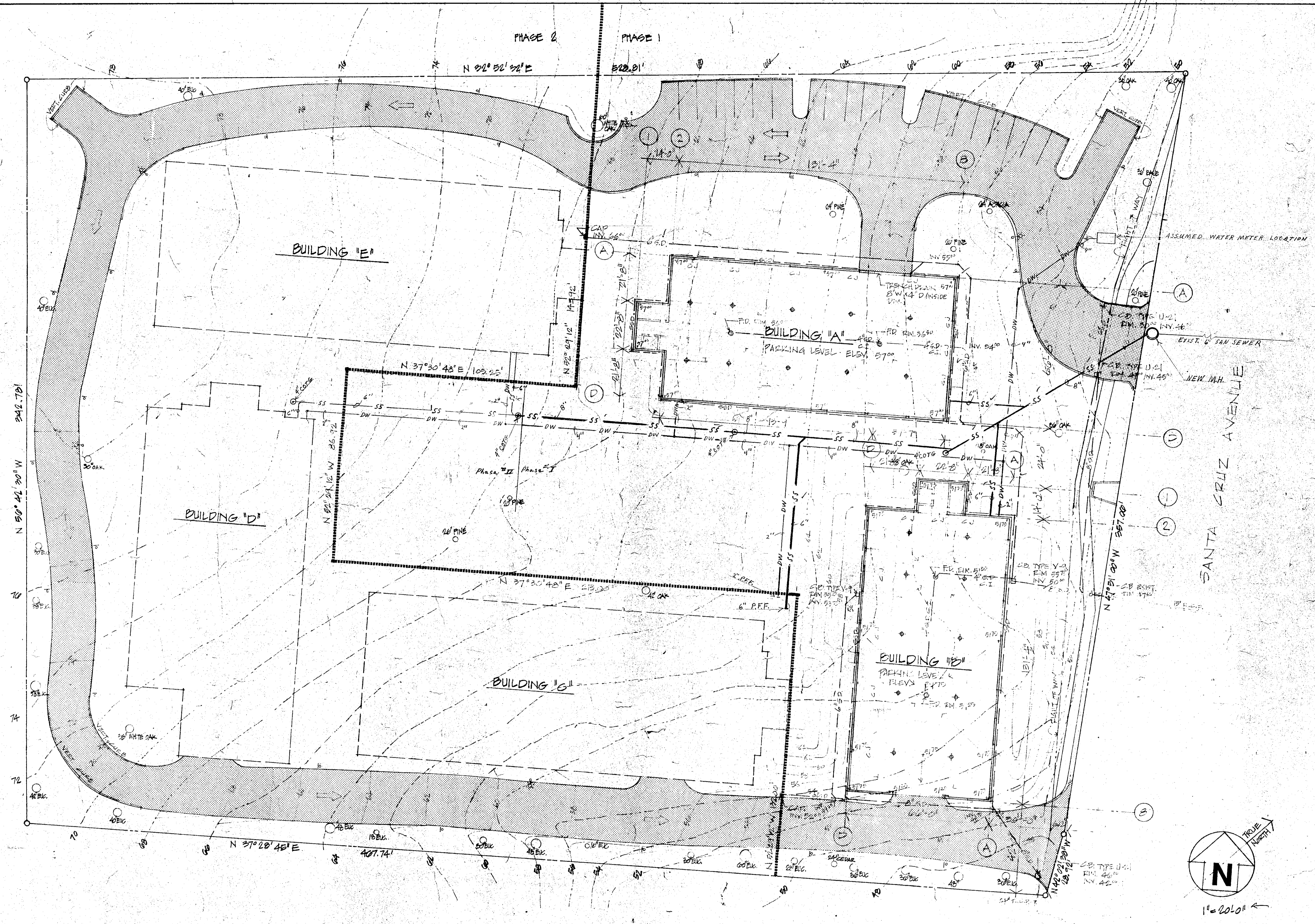
SITE PLAN
